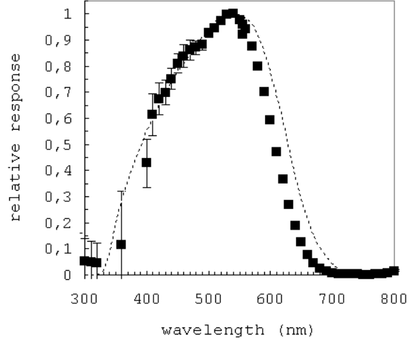
Fig. 9.— Measured SQM responsivity (squares) and calculated SQM responsivity (line).
