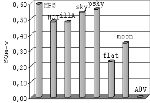
Fig. 14.— Conversion factors from SQM response to Johnson's V band.
