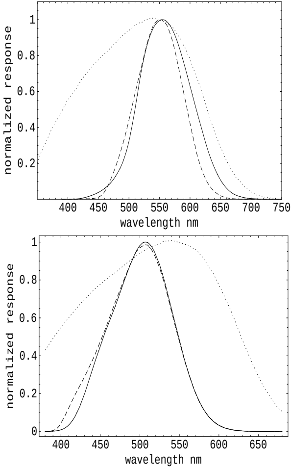
Fig. 21.— Top panel: CIE photopic response (solid line) and SQM + G28V filter (dashed line). Bottom panel: CIE scotopic response (solid line) and SQM + scotopic filter (dashed line).
