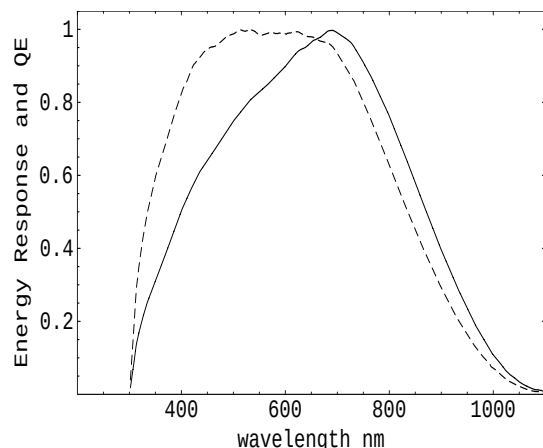
Fig. 7.— Normalized photodiode spectral responsivity (solid line) and quantum efficiency (dashed line).
