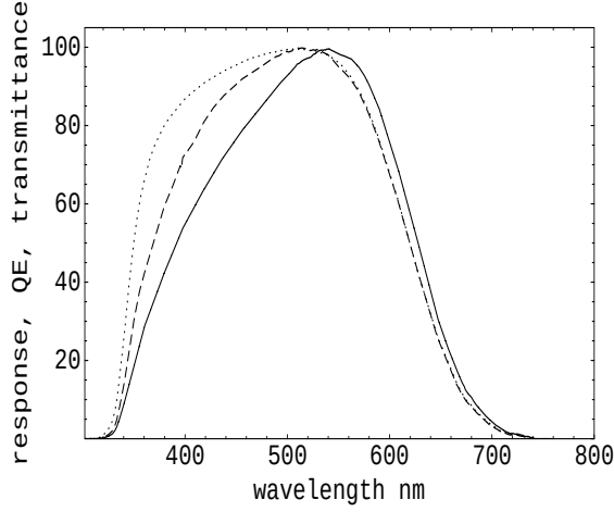
Fig. 8.— SQM normalized spectral responsivity (solid line), quantum efficiency (dashed line) and filter transmittance (dotted line).
