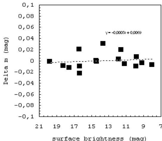
Fig. 6.— Residuals of the comparison of the SQM with a reference radiometer over a variable low-light calibration standard. They give an upper limit to linearity.
