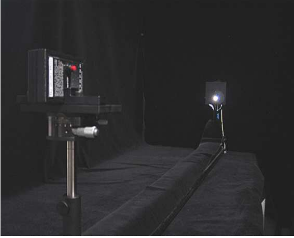
Fig. 1.— Measurement of the acceptance angle.
