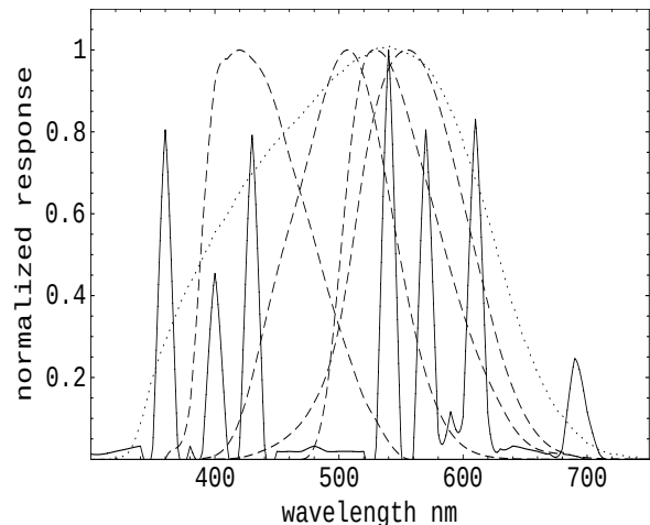
Fig. 12.— SQM normalized response (dotted line), standard normalized responses of Johnson's B band, CIE scotopic, Johnson's V band and CIE photopic (dashed lines from left to right) and emission spectra of an HPL mercury vapour lamp (solid line).
