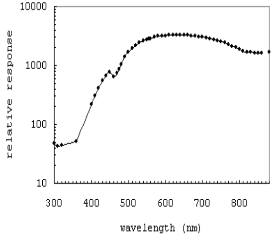
Fig. 10.— Response of the LPLAB's Low-Light-Level Spectral Responsivity Calibration Standard.
