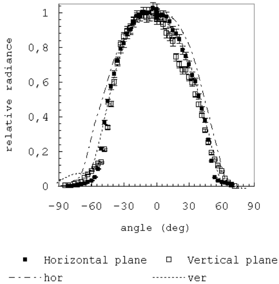
Fig. 3.— Angular response of SQM in a linear scale. Lines show the normalized output frequency of the detector at each angle provided by the detector manufacturer, along the vertical (dashed) and horizontal (dot-dashed) planes.
