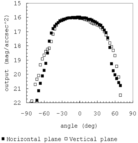
Fig. 2.— Angular response of SQM in magnitudes. Angles are positive downward and rightward.
