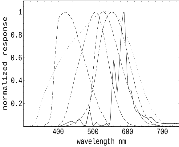
Fig. 13.— SQM normalized response (dotted line), standard normalized responses of Johnson's B band, CIE scotopic, Johnson's V band and CIE photopic (dashed lines from left to right) and emission spectra of an HPS High Pressure Sodium lamp (solid line).
