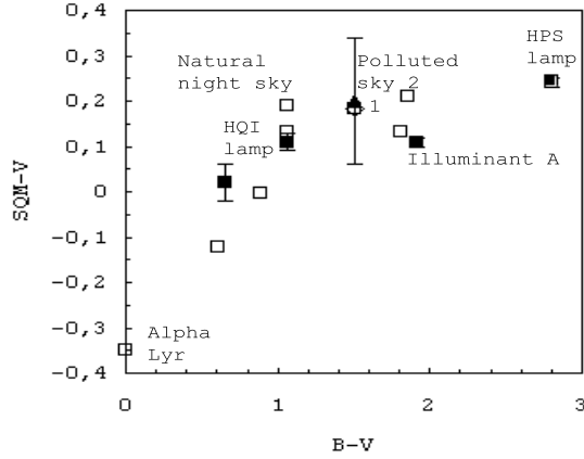
Fig. 15.— SQM-V measured ■ and calculated □.
